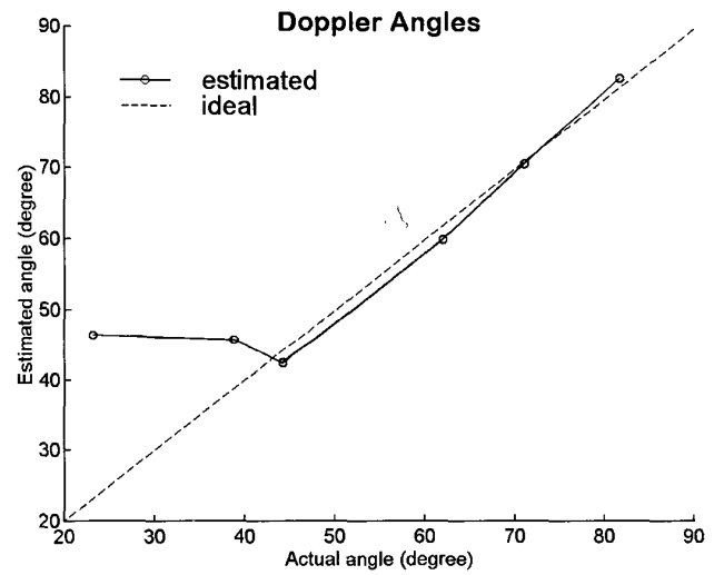
Fig. 11. Measured Doppler angles (solid with circles) vs. true Doppler angles (dashed): correlation.
