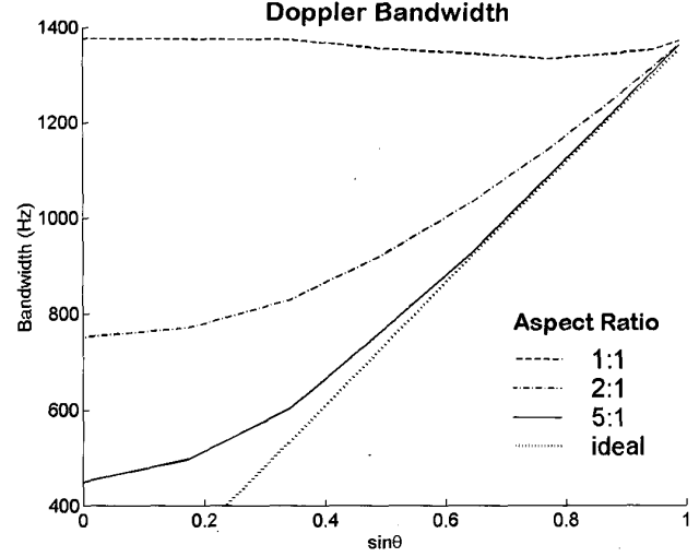
Fig. 2. Effects of aspect ratio on Doppler bandwidth.
